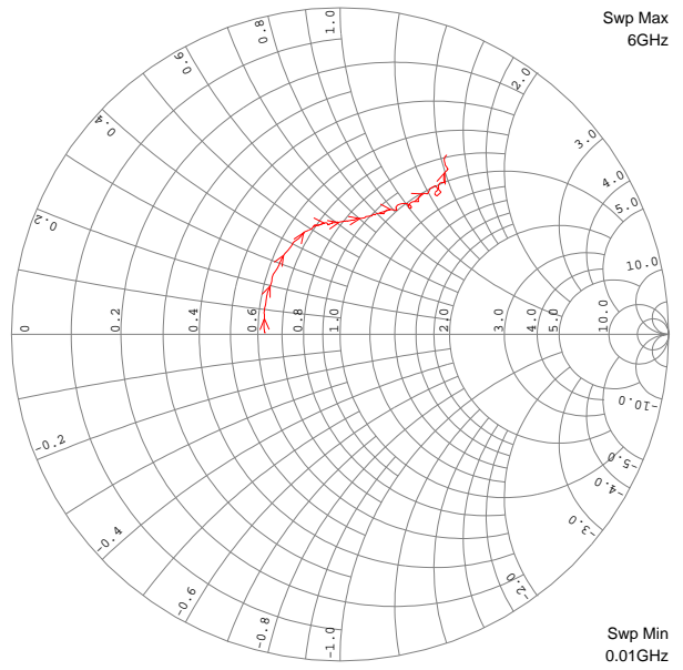
De-Embedded S22, V_{CC} = 3.67V , I_{CC} = 40mA , T = 25^{\circ}C
